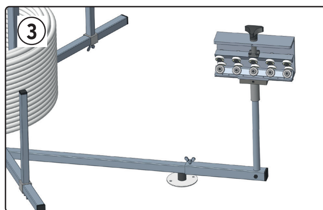
Adapter for pipe straightener
