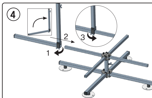
Slide the guide rod extension on and secure it.
