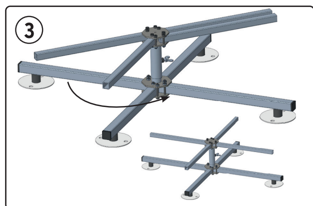
Position the outriggers at 45° intervals.
