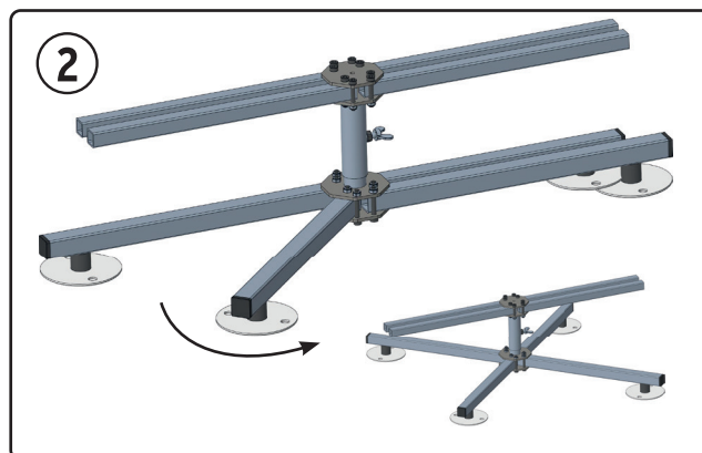
Position the support feet at 45° intervals.
