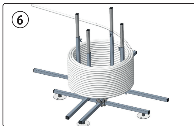
Mount the pipe coil and unwind the pipe end.
